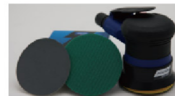
P3000精磨海绵Q255+ P2000T402精磨水砂
